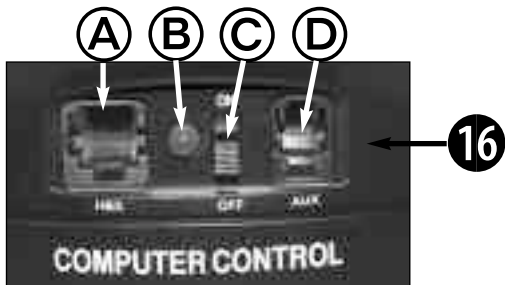
Fig. 1b : The computer control panel: A - HBX port; B - LED; C - On/Off; D - AUX port.
