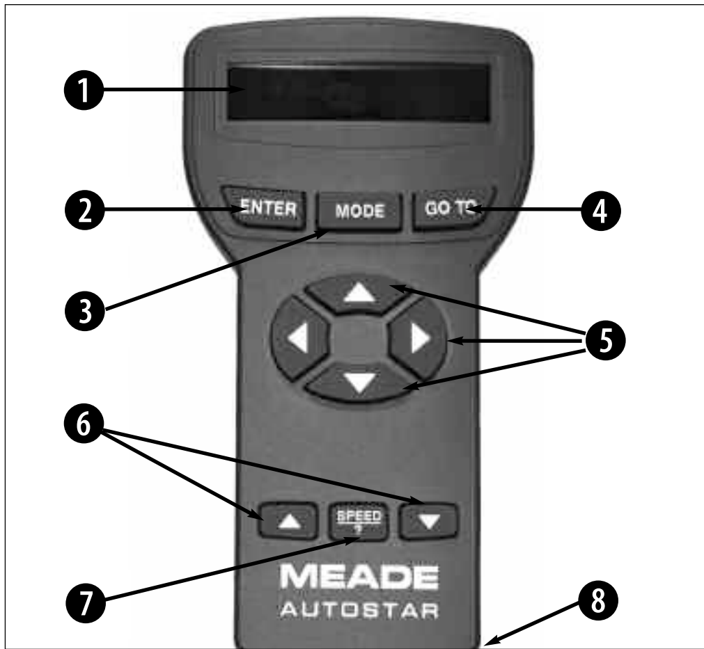
Fig. 5: #494 AutoStar Handbox.
