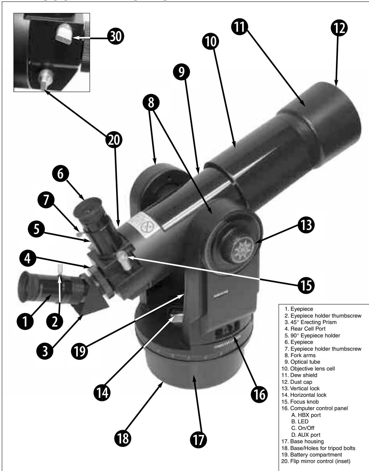
Fig. 1: The ETX-80AT-BB Telescope.
